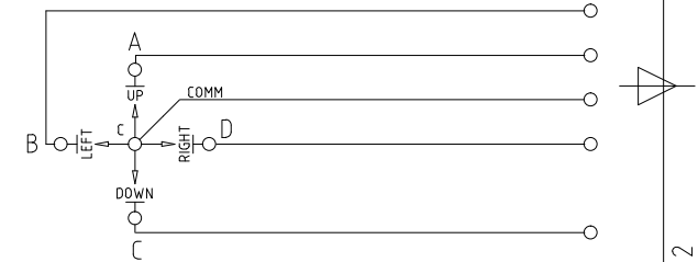
SCHEMATIC DIAGRAM
