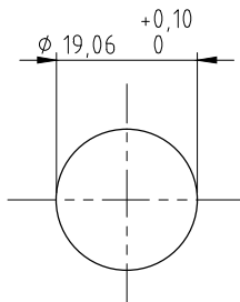
DETAIL PANEL HOLE SCALE 1:1
